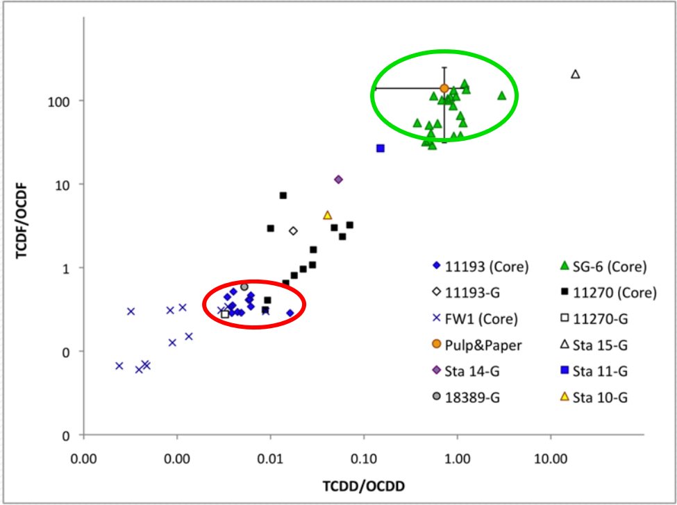
Literature values for pulp and paper endmember from Rappe et al., 1987 and MacDonald et al., 1998
