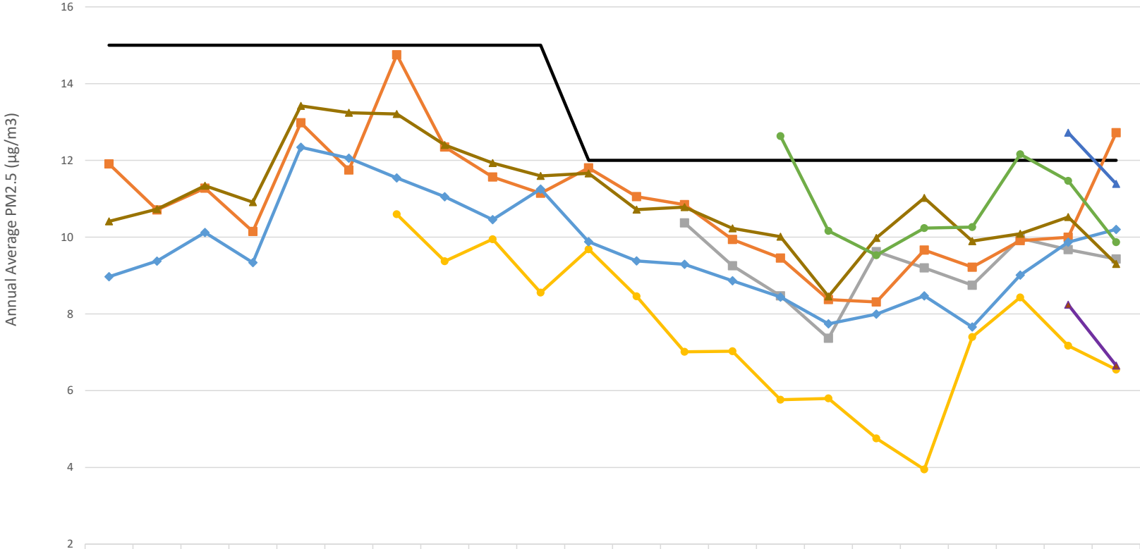
Annual Average PM2.5 (Local Conditions)
